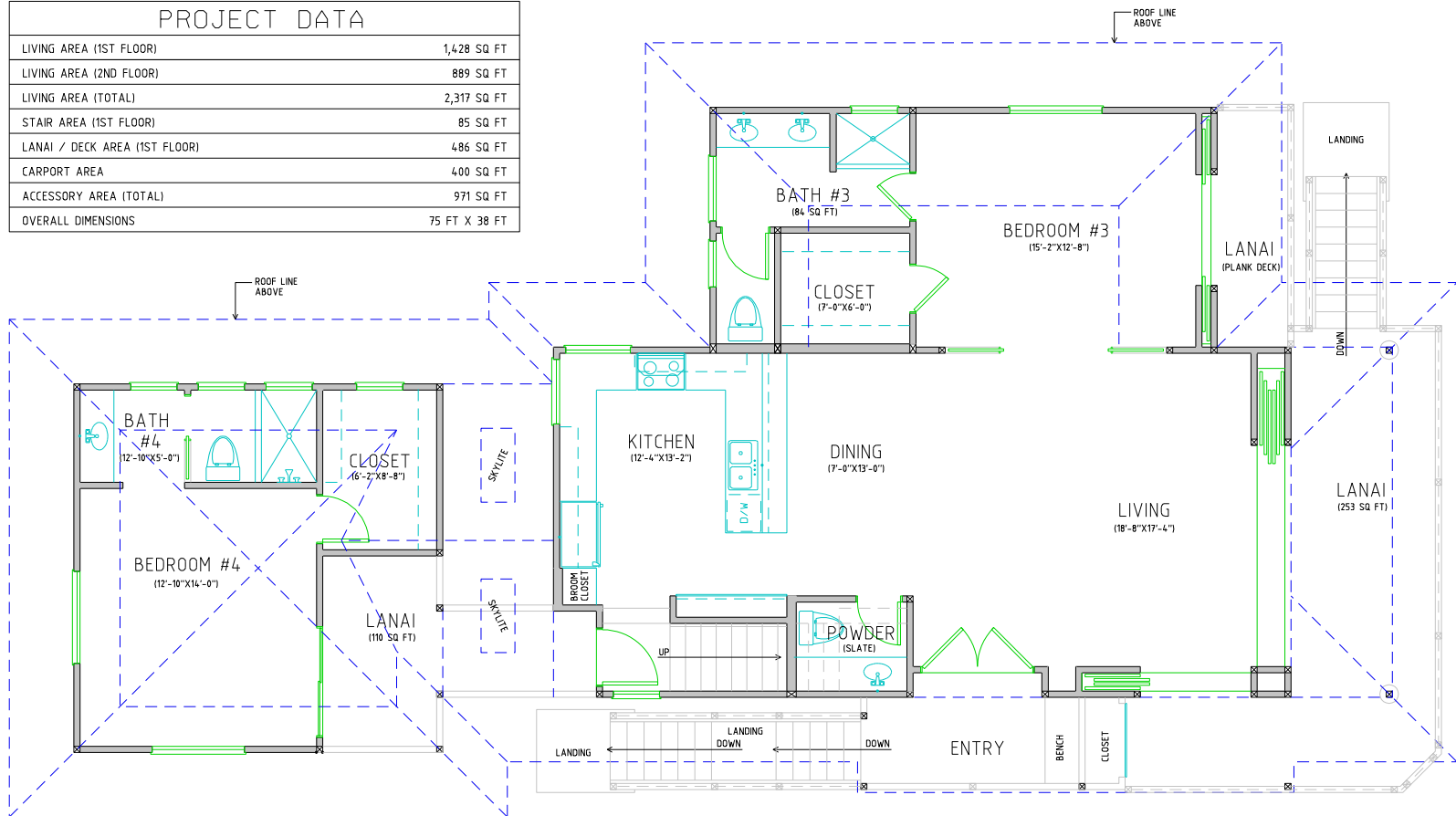
FLOOR PLAN - LYMAN'S BAY (1ST FLOOR)
